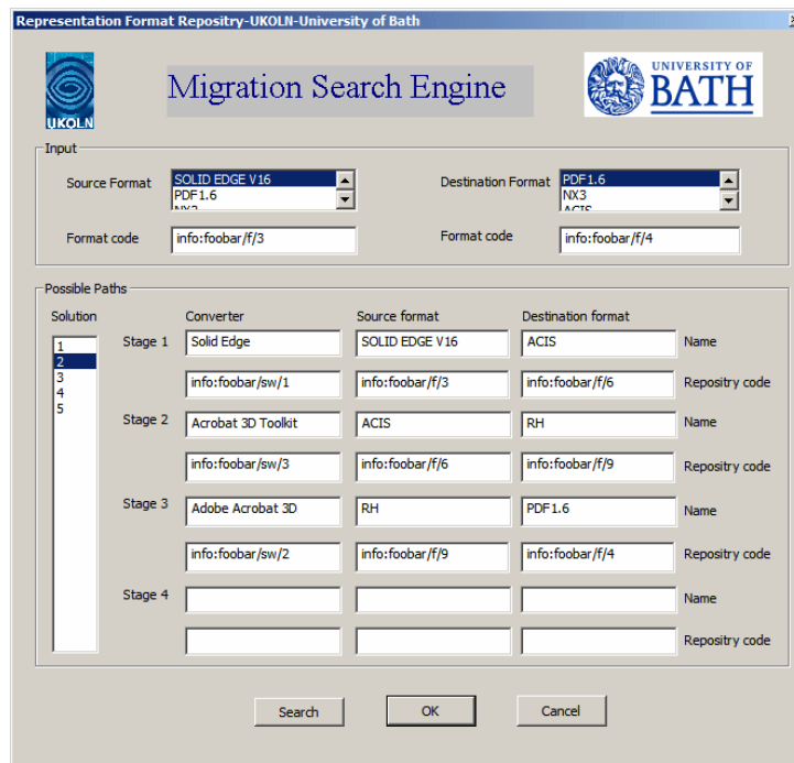
Figure 3 – The query interface for searching for migration paths between two formats, allowing a maximum of four migration stages.
